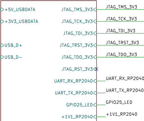
RP2040 for JTAG and UART
